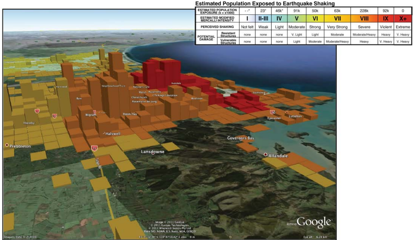
Figure 2: Christchurch Earthquake Population Exposure showing the extent of earthquake ground shaking (represented in colour) overlain on population density (represented as height of vertical bars) at a grid size of 1 km 2 . The colour key is based on the Mercalli scale, which is a measure of shaking, and explains how severe the ground shaking is for each colour. (Source: USGS)
